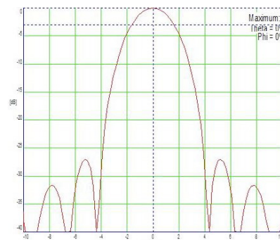
Antenna 10GHz 60cm
